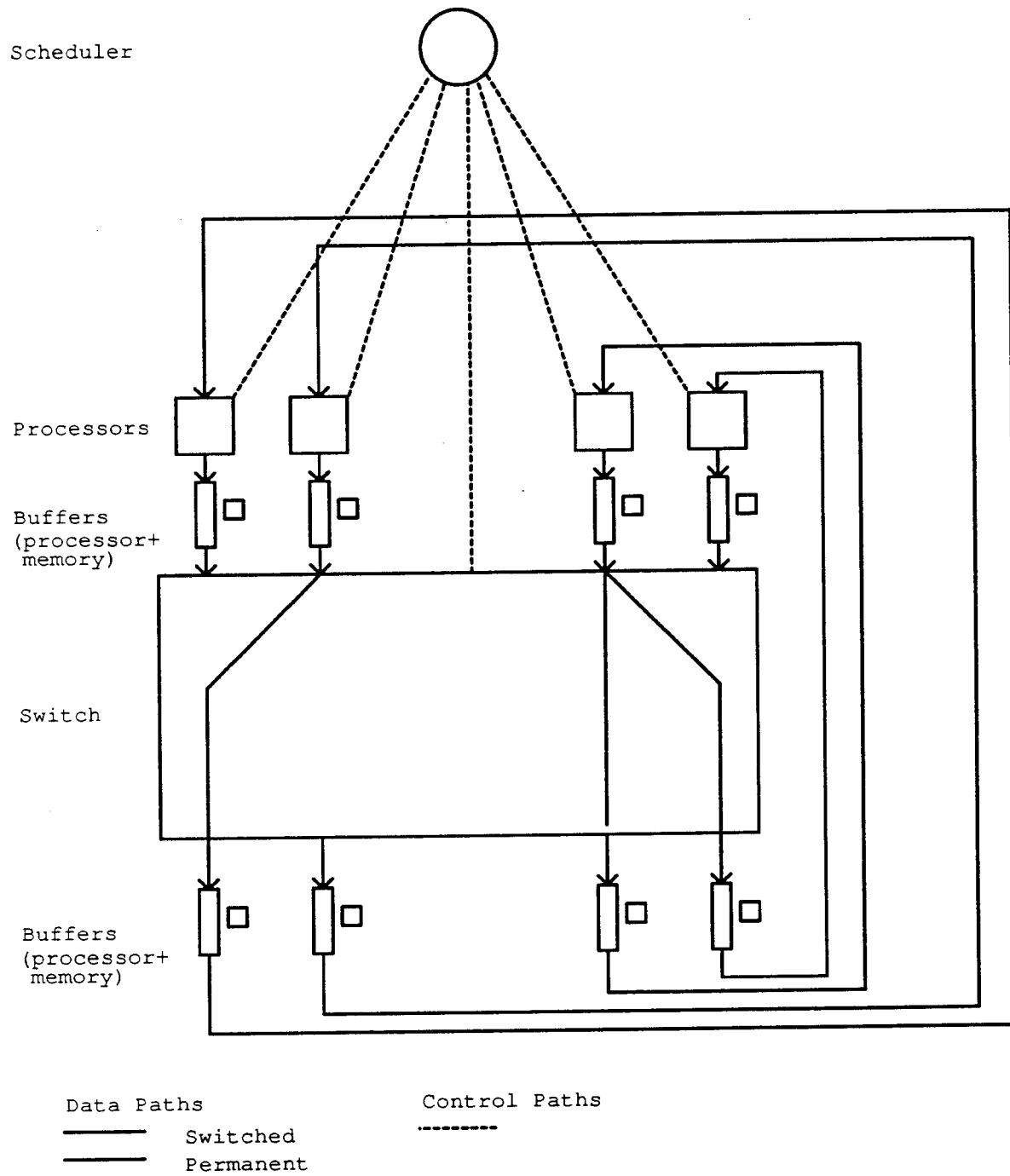
Figure 1 -- Physical Components
