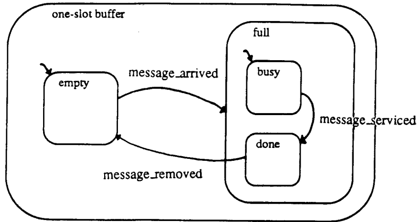
Figure 2: Statechart Specification of a One-Slot Buffer
