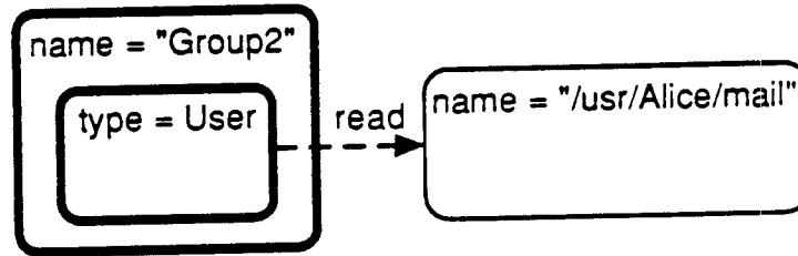
Figure 16: A composite constraint
