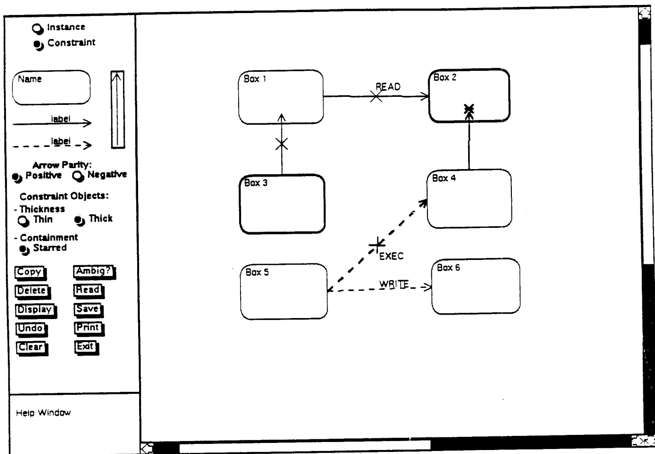
Figure 21: The Miró editor and a sample constraint picture
