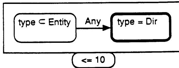
Figure 17: No directory may have more than 10 arrows pointing at it
