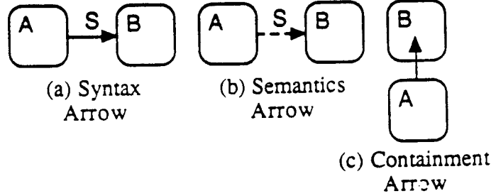
Figure 11: The three constraint arrows types
