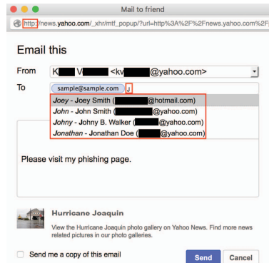
Fig. 4. Extracting contact list and sending email from the victim's account in Yahoo.
