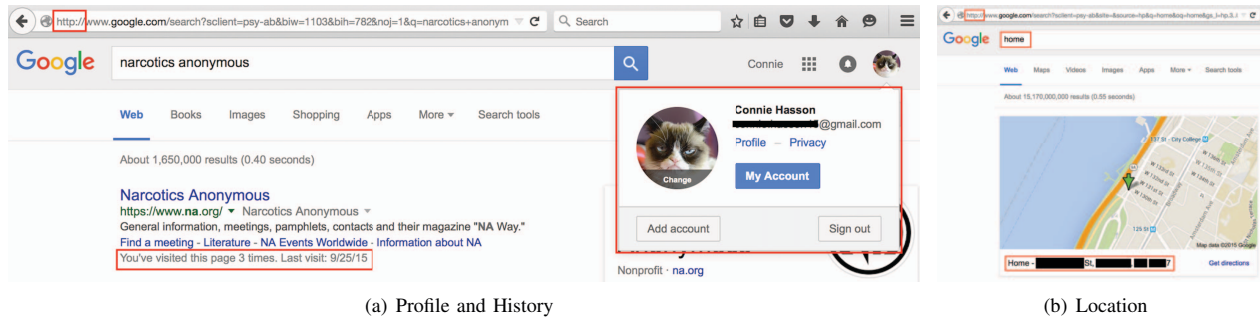
Fig. 3. Private information obtainable from user's Google account through HTTP cookie hijacking.
