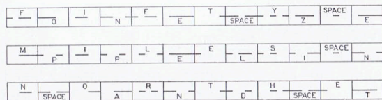
FIG. 5—TAPE RECORD OF MULTIPLEX PRINTER SIGNALS
