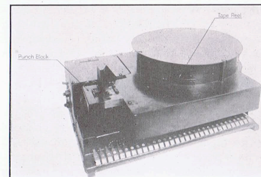
FIG. 10—MACHINE PERFORATOR
