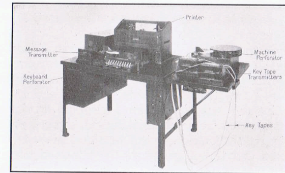
FIG. 1—CIPHER PRINTING TELEGRAPH MACHINE
