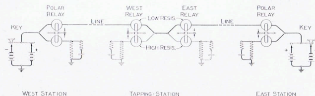
FIG. 4—METHOD OF TAPPING A DUPLEXED LINE
