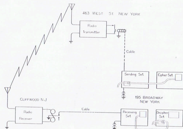
FIG. 11—Circuit for Radio Cipher Demonstrations
