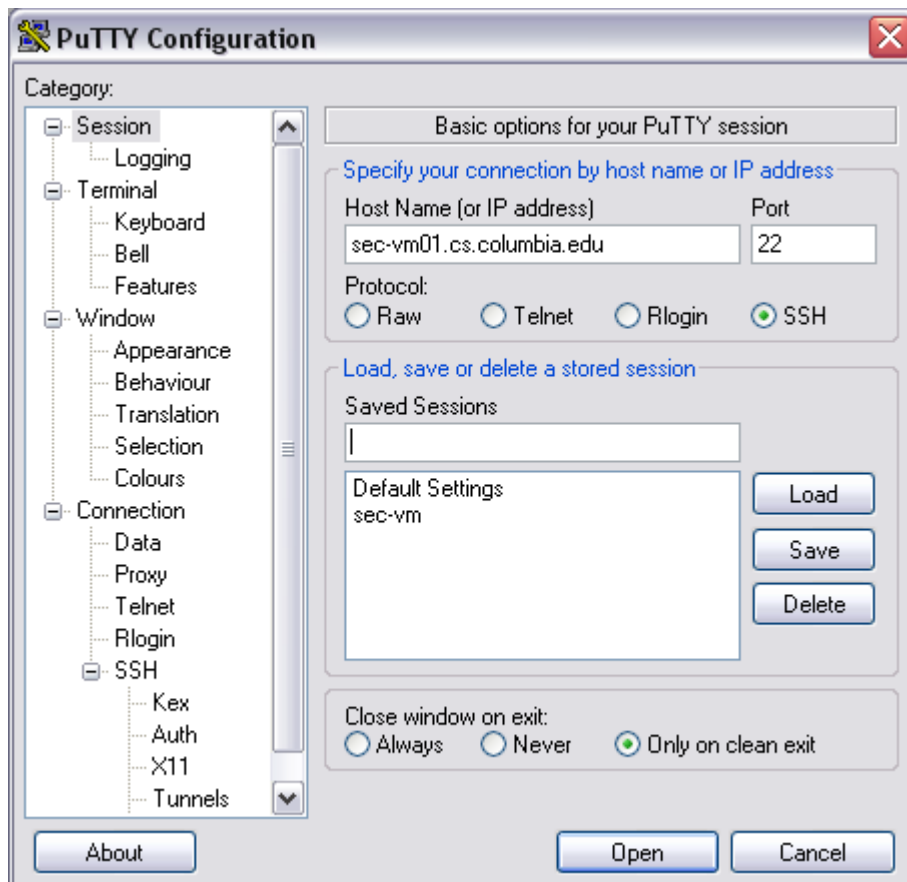
Figure 1: PuTTY Session Setup
