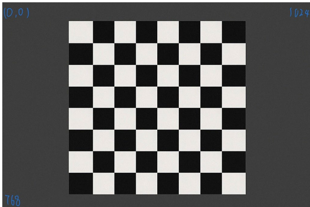
Figure 2. chessboard algorithm
