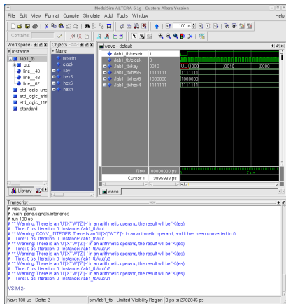
Figure 16: Running ModelSim and observing simulation results
