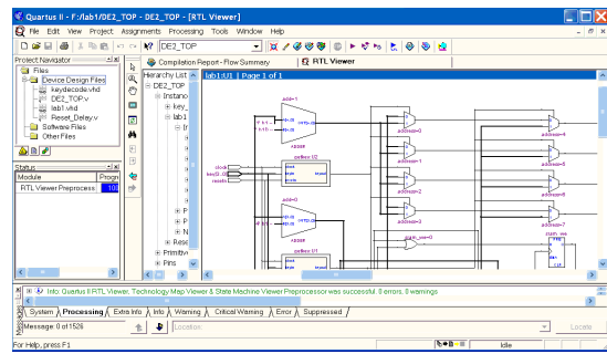
Figure 17: Viewing your design as a schematic
