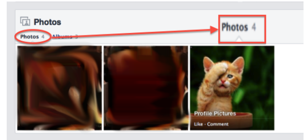
Fig. 1: An example of a side channel in Facebook. There are only three photos displayed. In contrast, Facebook lists that there are four photos in this photo album. Users viewing this can infer that one photo has been blocked from them by the user who posted these photos.
