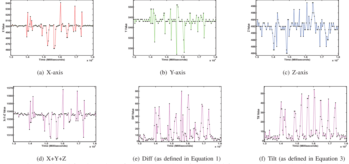
Figure 1. Plotted axis and function values of accelerometer data of tag, polled from computer through Alien reader interface for bit sequence ‘000110010101010100’ (here, ‘0’ encodes no-vibration and ‘1’ encodes vibration)
