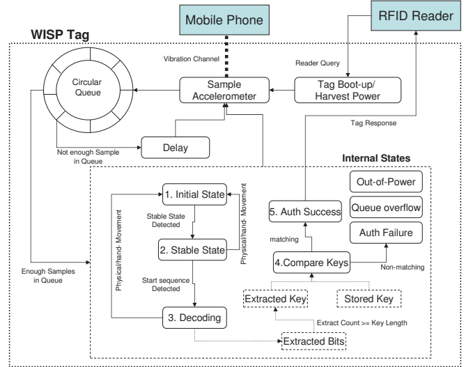
Figure 2. Block Diagram of Vibration Decoding and Authentication Algorithm on WISP Tag
