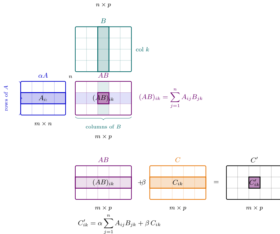
Figure 1: Diagram of a GEMM C \leftarrow \alpha AB + \beta C . A sits left of AB (same m rows) and B sits above AB (same p columns); the inner dimension n meets at the corner and is summed out. The second row accumulates into the existing matrix C .
