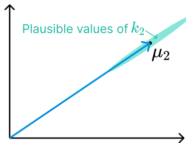
Figure 1: The vector \mu_2 (shown here in 2D as an example), with the range of possible values of k_2 shown in green. k_2 points in the same direction as \mu_2 , but may have larger or smaller magnitude.
