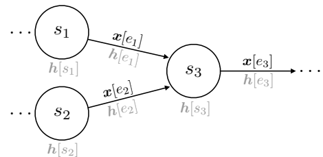
Figure 2: This example shows part of a lattice, with the RNN hidden representations shown in gray. \mathbf{h}[e_1] is computed based both on local arc features \mathbf{x}[e_1] and the representation \mathbf{h}[s_1] of the arc's source state (see Alg. 1, line 9); likewise for \mathbf{h}[e_2] . State representation \mathbf{h}[s_3] is computed by pooling the incoming arc representations \mathbf{h}[e_1] and \mathbf{h}[e_2] (see Alg. 1, line 13).
