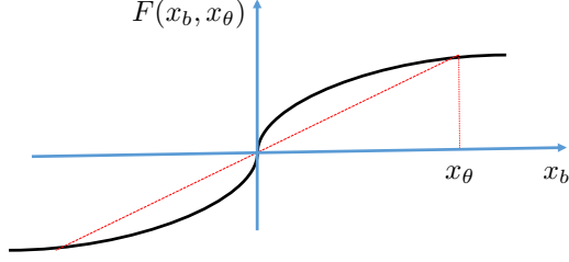
Figure 1: F(x_b, x_\theta) as a function of x_b when x_\theta is fixed. The black line represents the curve of function F and red line represents the diagonal line: y = x .
