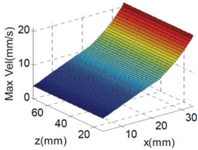
Fig. 8. Minimal joint velocity for parallelogram to carry out 30 mm/s velocity.
