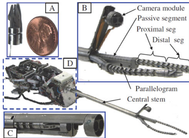
Fig. 1. IREP robot has two dexterous arms and a controllable stereo vision module. (a) Gripper and distal wrist. (b) IREP distal end in a working configuration. (c) IREP in a closed configuration (bottom shell cover removed). (d) Modular actuation unit of the IREP.
