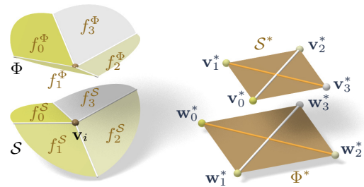
Figure 4: Mean curvature of a vertex \mathbf{v}_i of S : Corresponding edges of the polar duals S^*, \Phi^* are parallel, and mean curvature according to [Pottmann et al. 2007] is computed from the vertices polar to faces adjacent to \mathbf{v}_i . For valence 4 vertices the case of zero mean curvature shown here is characterized by parallelity of non-corresponding diagonals of corresponding quads in S^*, \Phi^* .
