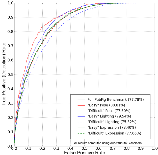
Figure 8: Face Verification Results on PubFig: Our performance on the entire benchmark set of 20,000 pairs using attribute classifiers is shown in black. Performance on the pose, illumination, and expression subsets of the benchmark are shown in red, blue, and green, respectively. For each subset, the solid lines show results for the “easy” case (frontal pose/lighting or neutral expression), and dashed lines show results for the “difficult” case (non-frontal pose/lighting, non-neutral expression).
