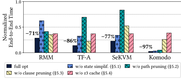
Figure 10. Ablation study of Spoq2 optimizations.
