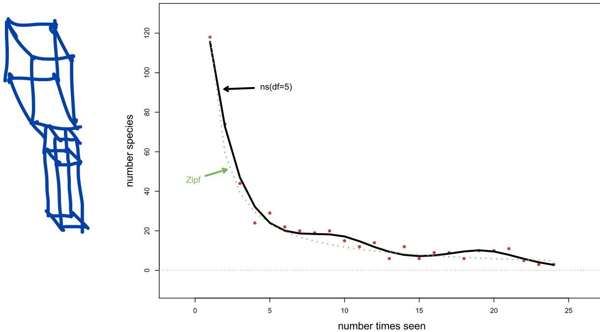
FIG. 4. Corbet's butterfly data. Red points are the (x, y) data from Table 3; solid black curve is natural spline Poisson regression fit, 5 degrees of freedom (57). Light green dashed curve follows Zipf's law: \hat{y}_x = y_1/x .
