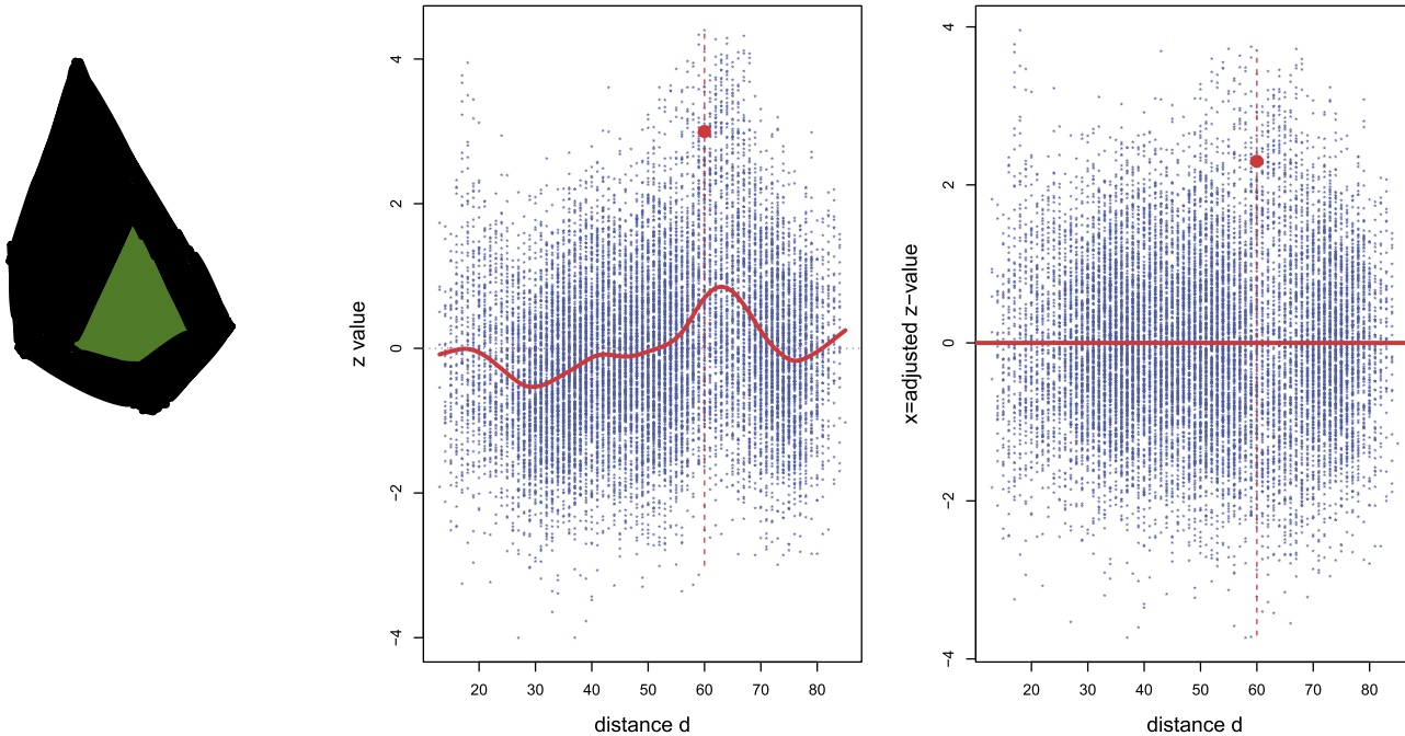
FIG. 13. DTI data. Left panel: z -values z_i plotted vertically versus voxel distance from back of the brain d_i ; red curve c(d) is smoothing spline, df = 13 ; large red dot (d_0, z_0) = (60, 3.0) . What is the posterior distribution of \delta_0 , the expectation of z_0 ? Right panel: Vertical axis is x_i = z_i - c(d_i) ; now the red dot at d_0 = 60 , x_0 = 3.0 - 0.7 = 2.3 . The expectation of x_0 is \theta_0 = \delta_0 - 0.7 .
