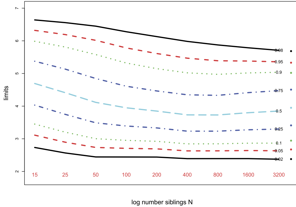
FIG. 11. Smoothed posterior percentiles 2%, 5%, ..., 98% of corrected estimates \tilde{g}(\theta_0 | x_0 = 5) based on first N siblings, gamnormal example, as N increases. Points at extreme right are percentiles of true posterior g(\theta_0 | x_0 = 5) for \theta \sim \text{Gamma}_9/3 . See Remark H.
