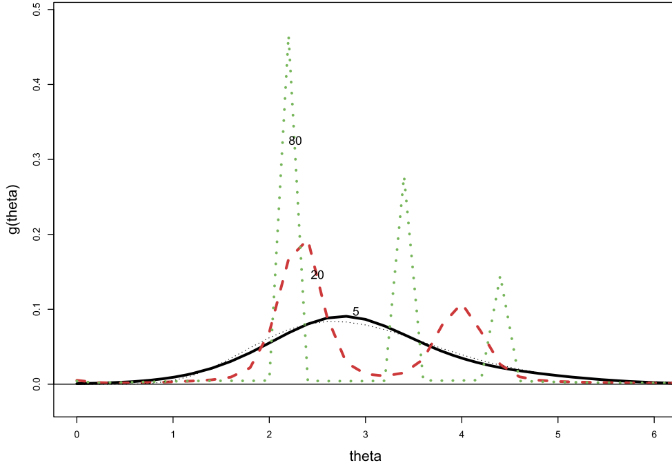
FIG. 12. Prior density estimates \hat{g}(\theta) based on all N = 3200 gamnormal observations. For natural spline g -models and degrees of freedom 5, 20, and 80. Light black dotted curve is the true prior density \text{Gamma}_9/3 .
