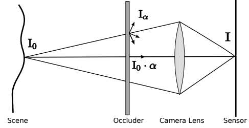
Figure 2: Image formation model: \alpha \in [0, 1] is the attenuation pattern of the intermediate layer, i.e., the fraction of light transmitted ( 0 = completely blocked). The camera is focused on the target scene. The final image \mathbf{I} is the sum of the attenuated light from the background after the defocus blur, \mathbf{I}_0 \cdot (\alpha * \mathbf{k}) , and the light emitted from the intermediate layer itself, \mathbf{I}_\alpha * \mathbf{k} .
