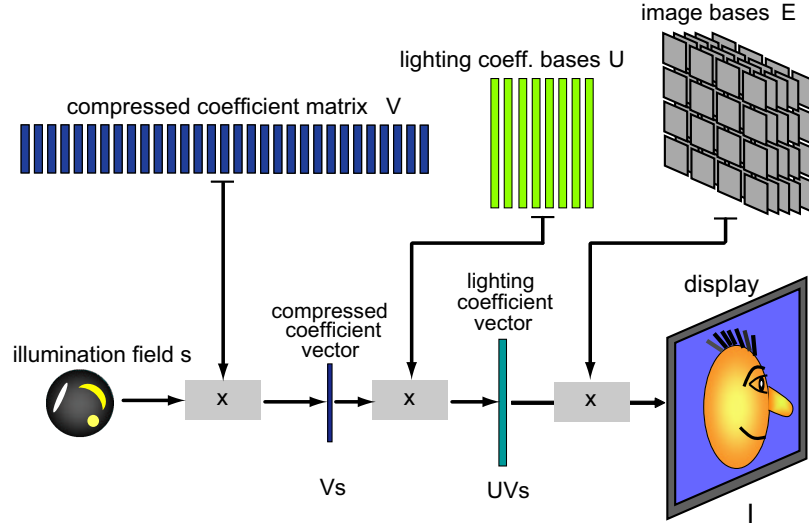
Fig. 7. To render an image of the scene as if it were illuminated by a field specified by a vector s we appeal to the previously calculated matrices E , U and V . First, we compute a compressed coefficient vector as the product Vs . Next, we compute a lighting coefficient vector as the product UVs . Note that the vector UVs has dimension (m \times b) \times 1 and that the subvector l^j given by the rows b \times (j - 1) + 1 through b \times j of UVs contain the coefficients necessary for rendering the j th block. Thus, the subvectors can be unstacked and used to render the j th block of the displayed image as the product E^j l^j . This process is repeated for all m blocks and an image is displayed on completion.
