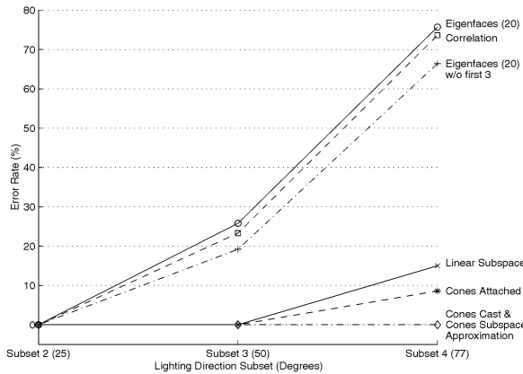
Fig. 12. Extrapolation in Illumination: Each method was trained on seven images per person from Subset 1 (near-frontal illumination), Pose 1 (frontal pose). The plots show the error rates under more extreme lighting conditions while the pose was kept fixed. The experiments were conducted on 450 images from Pose 1.
