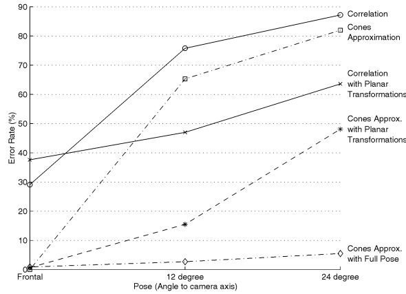
Fig. 13. Extrapolation in Pose: Error rates (%) as the viewing direction becomes more extreme. The five methods have been trained on seven images per person from Subset 1 (near-frontal illumination), Pose 1 (frontal pose). Note that each reported error rate is for all illumination subsets (1 through 4). The “Frontal Pose” includes 450 test images, the “12 degree” (Poses 2, 3, 4, 5, 6) includes 2,250 test images, and the “24 degree” (Poses 7, 8, 9) includes 1,350 test images.
