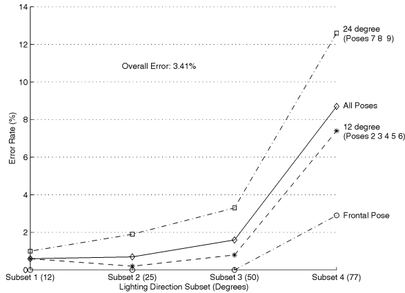
Fig. 14. Error rates (%) for different poses against variable lighting using our face representation proposed in Section 3. The training was performed on seven frontal-pose images per face with near-frontal illumination. The tests were conducted on a total of 4,050 images of 10 faces from all nine poses of the Yale Face Database B.
