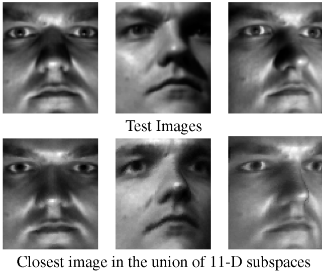
Fig. 9. Top Row: Three images of a face from the test set. Bottom Row: The closest reconstructed images from the representation proposed in Section 3. Note that these images are not explicitly stored or directly synthesized by the generative model, but instead lie within the closest matching linear subspace.
