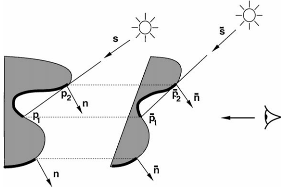
Figure 3. The image points that lie in shadow for a surface under light source \mathbf{s} are identical to those in shadow for a transformed surface under light source \tilde{\mathbf{s}} = G\mathbf{s} . In this 2-d illustration, the lower shadow is an attached shadow while the upper one is composed of both attached and cast components. A generalized bas relief transformation with both flattening and an additive plane has been applied to the left illustration, yielding the right one. For diagrammatic clarity, the surface normals are drawn outward.
