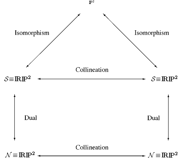
Figure 4. The relationship of different spaces in proof of Proposition 4.
