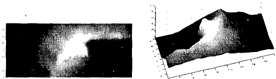
Figure 1: The measured intensity of one pixel as a function of light source position. Images were acquired as a point source was moved over a quarter of a sphere.
