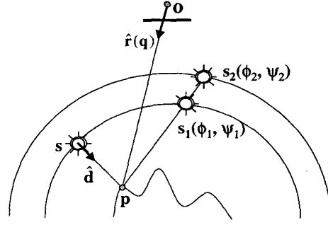
Figure 5: A 2-D schematic of the reconstruction setup. A camera whose origin is at \mathbf{o} observes a scene point \mathbf{p} which is illuminated by light sources covering two surfaces, parameterized as \mathbf{s}_1(\phi_1, \psi_1) and \mathbf{s}_2(\phi_2, \psi_2) .
