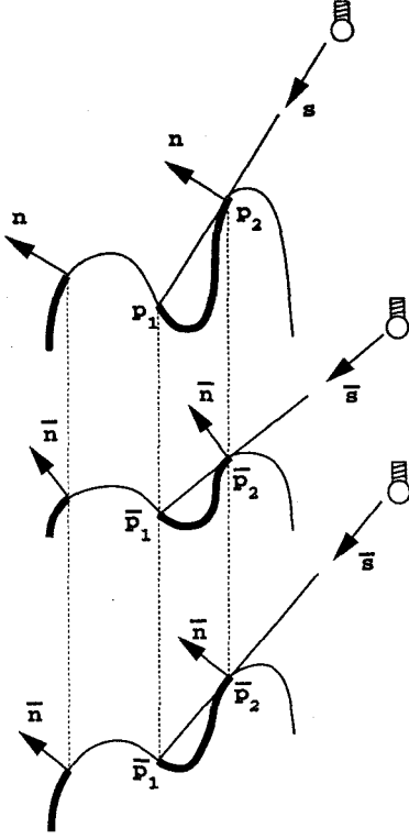
Figure 2: The image points that lie in a cast or attached shadow for a surface f under light source s are identical to those in shadow for transformed the surface \tilde{f} under light source \bar{s} = G^{-T}s . The middle figure shows a classical bas-relief transformation of the upper figure while the bottom figure is a generalized bas-relief. For diagrammatic clarity, the surface normals are drawn outward.
