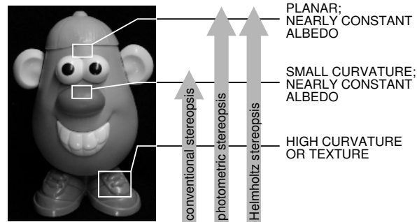
Fig. 4. A summary of the surface properties required for Lambertian surface reconstruction by conventional, photometric and Helmholtz stereo techniques. Even when the BRDF is Lambertian, conventional stereopsis is only capable of recovering surface geometry in regions of texture (i.e. varying albedo) or high curvature (i.e. edges). Neither photometric stereopsis nor Helmholtz stereopsis suffer from this limitation.
