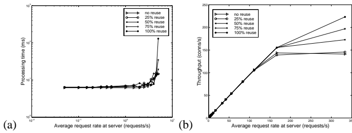
Figure 16: Effect of session reuse rate on the server processing times (a) and the server throughput (b).
