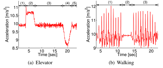
Fig. 6. Acceleration of elevator and walking.
