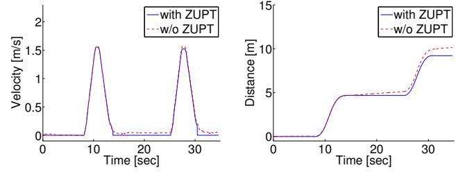
Fig. 2. Velocity and distance calculations with and without ZUPT.
