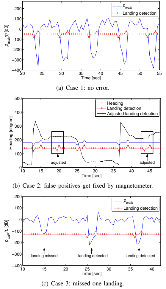
Fig. 4. Three landing detection cases.
