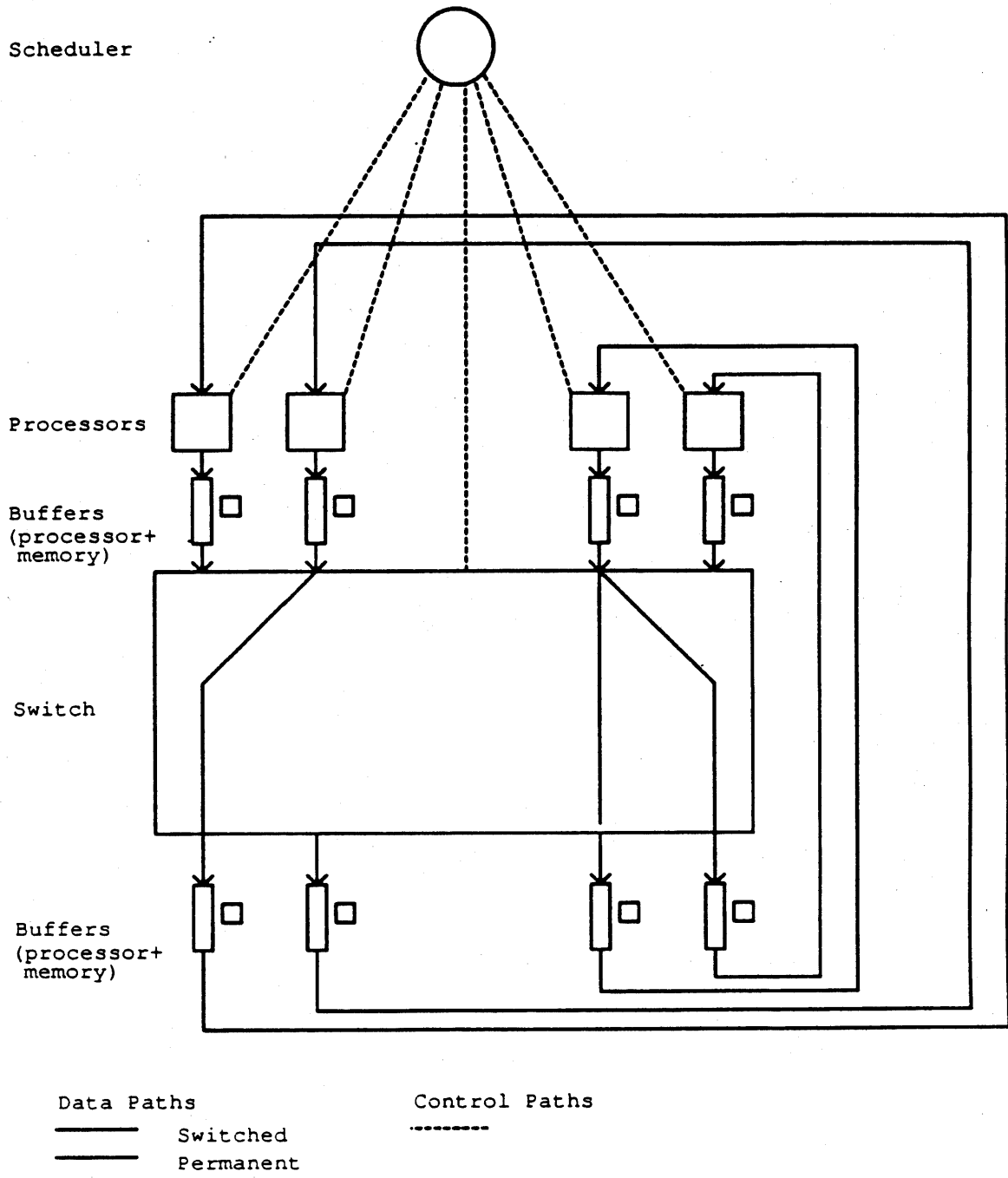
Figure 1 -- Physical Components
