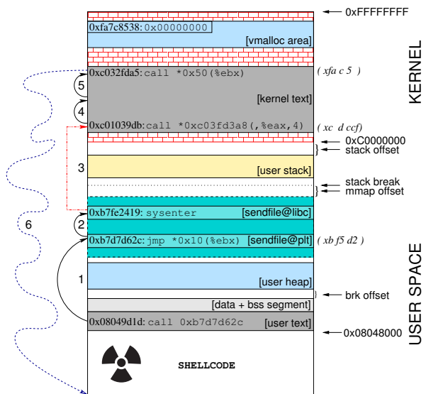
Figure 5: Control transfers that occur during the exploitation of a ret2usr attack. The sendfile system call, on x86 Linux, causes a function pointer in kernel to become NULL , illegally transferring control to user space code.
