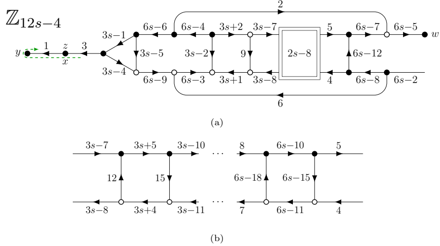
Figure 2: The fixed part of the current graph (a) contains the salient currents for adding one handle, and the simple ladder (b) inside the box. The label on the box indicates the number of “rungs” in the ladder, whose orientations alternate and whose currents form an arithmetic sequence.
