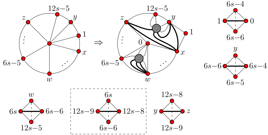
Figure 3: The embedding near vertex 0 is augmented using a handle, which is represented by excising two disks and identifying their boundaries. For the edge flips, the dashed edges are replaced by the thick solid edges. The quadrilateral inside the box has the reverse orientation for s = 3 .
