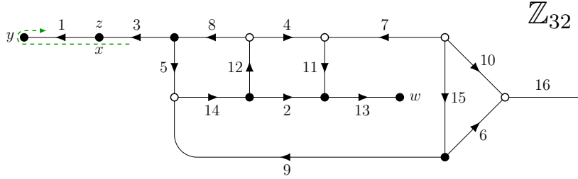
Figure 1: An index 1 current graph with current group \mathbb{Z}_{32} generating a triangular embedding of K_{36} - K_4 . Solid and hollow vertices represent clockwise and counterclockwise rotations, respectively.
