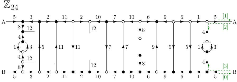
Figure A.1: This index 4 current graph, which generates a triangular embedding of K_{24} , was discovered using techniques found in Pengelley and Jungerman [PJ79]. The ends labeled “A” and “B” are identified to form a cylindrical digraph.
