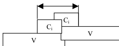
Figure (4) Gestures in a VC_i\#C_iV with stiffness k .
