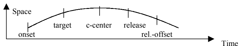
Figure (1) Spatio-temporal realization of a gesture.
