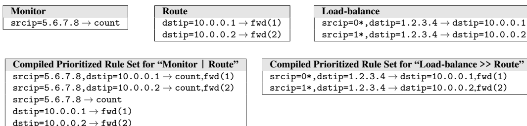
Figure 1: Parallel and Sequential Composition.
