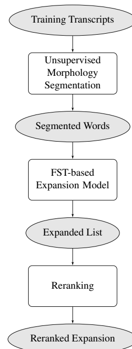
Figure 1: The flowchart of the lexicon expansion system.
