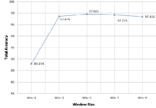
Fig. 1. Ezafe Recognition Accuracy vs. Window Size
