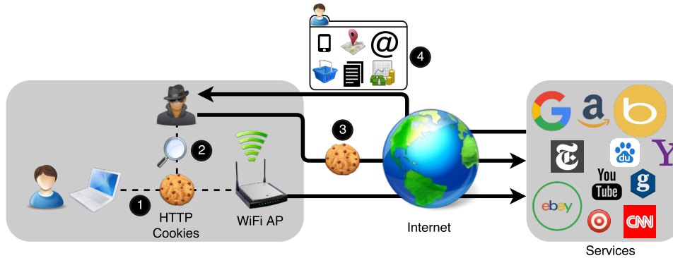
Fig. 1. Workflow of an HTTP cookie hijacking attack. After the victim’s cookies are exposed on the unencrypted connection (1) and stolen (2), the attacker can append the stolen cookies when browsing the target websites (3) and gain access to the victim’s personal information and account functionality (4).
