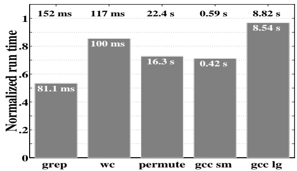
Figure 8: Various application runtimes
