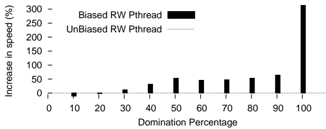
Figure 16: A comparison of our biased rwlock with Linux thread rwlock.
