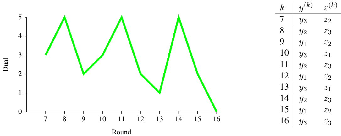
Figure 15: Figures showing progress of the subgradient algorithm for f(y) = [1, 1, 2] and g(z) = [1, 1, -2] , with the additional constraint y(1, a, b) = z(1, a, b) incorporated in the Lagrangian. The graph shows the dual value L(u^{(k)}) versus number of iterations k . The table shows the hypotheses y^{(k)} and z^{(k)} versus number of iterations k .
