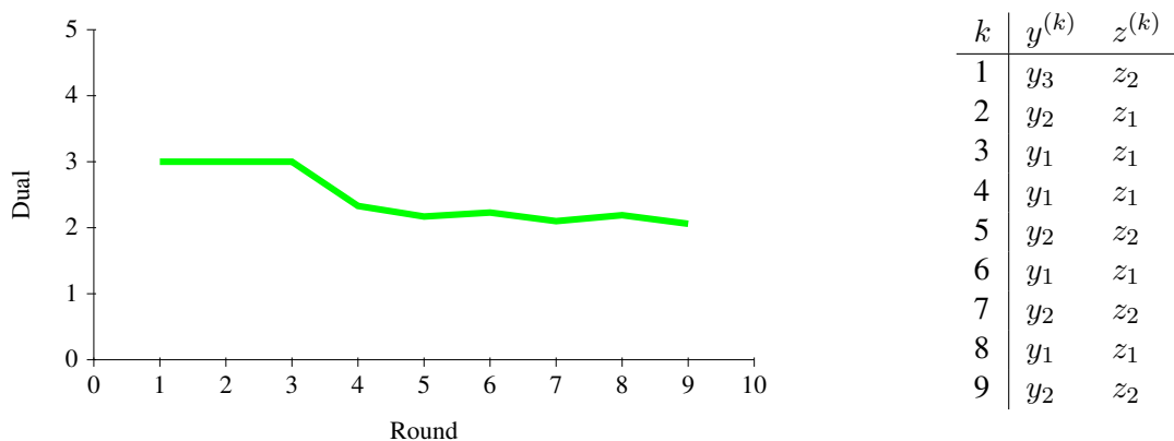
Figure 14: Figures showing progress of the subgradient algorithm for f = [1, 1, 2] and g = [1, 1, -2] . The graph shows the dual value L(u^{(k)}) versus number of iterations k . The table shows the hypotheses y^{(k)} and z^{(k)} versus number of iterations k . In later iterations the method alternates between hypotheses (y_1, z_1) and (y_2, z_2) .
