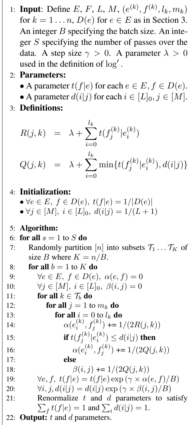
Figure 5: The stochastic exponentiated-gradient algorithm for optimization of I2CR-2.
