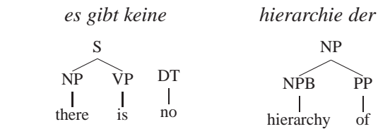
Figure 2: Example syntactic phrase entries. We show German sub-strings above their associated sequence of treelets. 4
