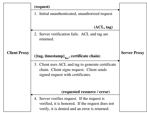
Figure 4: SPKI/SDSI Proxy to Proxy Access Control Protocol
