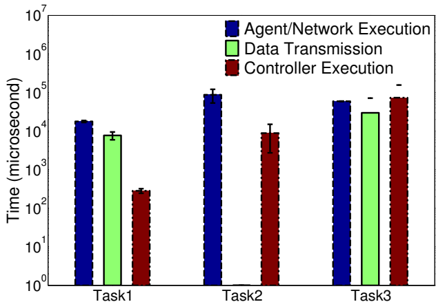
Figure 7: Breakdown of execution latency
