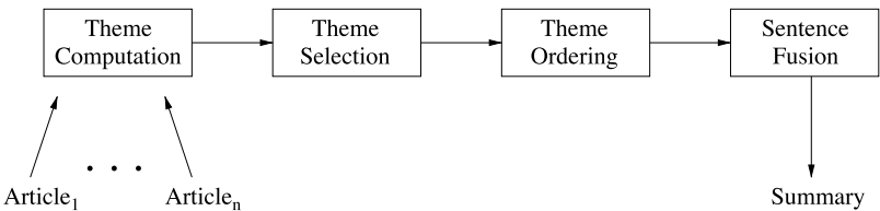
Figure 2 MultiGen architecture.
