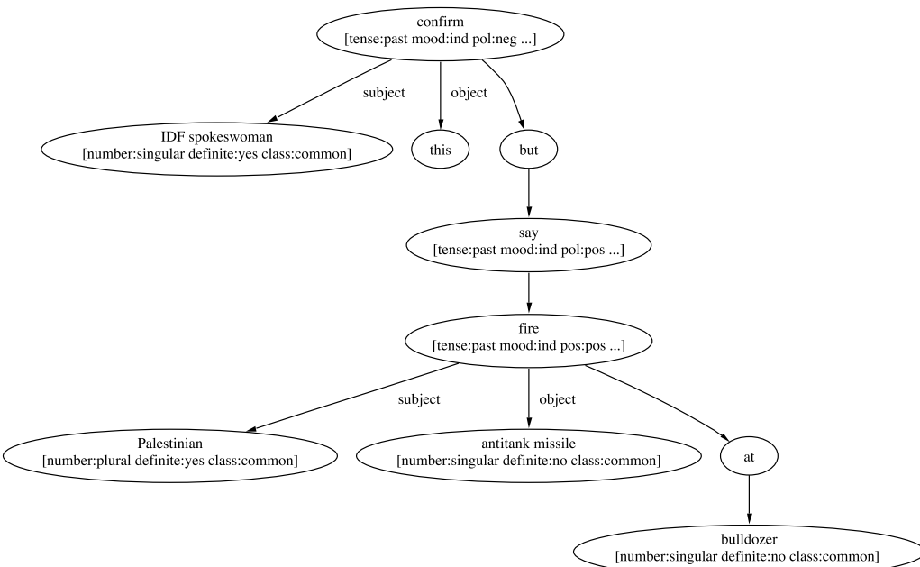
Figure 3 Dependency tree of the sentence The IDF spokeswoman did not confirm this, but said the Palestinians fired an antitank missile at a bulldozer on the site. The features of the node confirm are explicitly marked.
