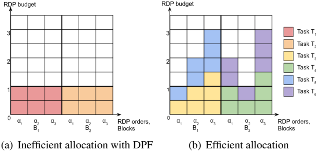
Fig. 3. Example of allocations with RDP accounting. In Fig. 3(a), DPF treats RDP orders like a regular resource and orders tasks by dominant share, allocating only 2 tasks in this example. Meanwhile, Fig. 3(b) leverages the fact that only one order per block has to be below the capacity (here, \alpha_1 for block B_1 and \alpha_2 for block B_2 ). Tasks T_3 and T_5 have a large dominant share of 1.5 but are efficient because they request only 0.5 for B_1 's best alpha, \alpha_1 .
