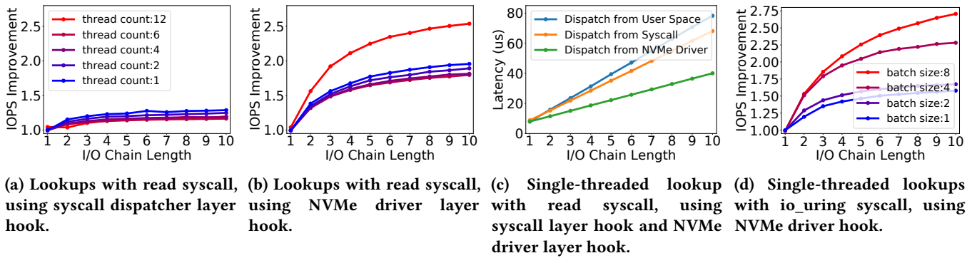
Figure 3: Search throughput improvement on B-tree with varying depth when reissuing lookups from different kernel layers.
