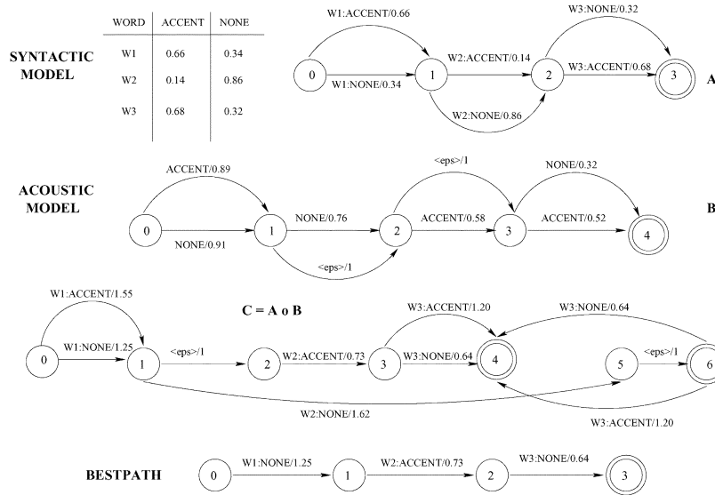
Fig. 2. Illustration of the FST composition of the syntactic and acoustic lattices and resulting best path selection. The syntactic–prosodic maxent model produces the syntactic lattice and the HMM acoustic–prosodic model produces the acoustic lattice.
