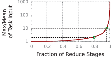
Figure 6: Skewness
