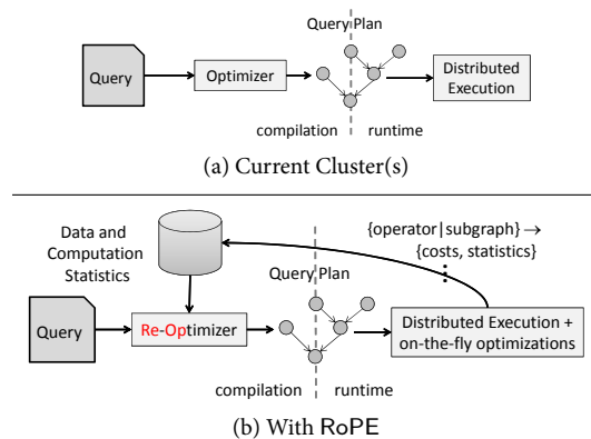
Figure 9: RoPE’s architecture for re-optimization
