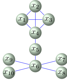
Figure 10: ‘Lamp’ topology. maxW is likely to choose x_6 since it has the highest degree, but x_4 is typically a better choice since it lies on cycles. Mpover can recognize this and make a better choice.
