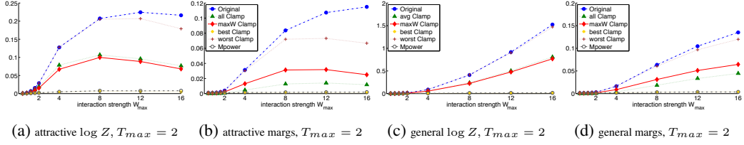
Figure 11: Average errors vs true, ‘lamp’ topology T_{max} = 2 . Consistent legend throughout. Mpower performs well, significantly better than maxW.
