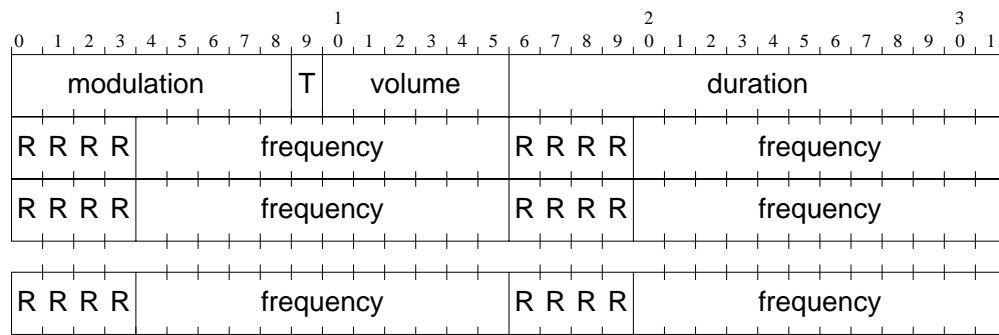
Figure 2: Payload format for tones
