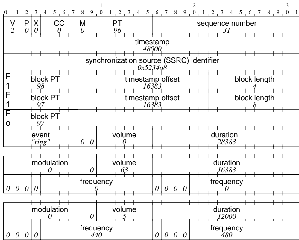
Figure 3: Combining tones and events in a single RTP packet
